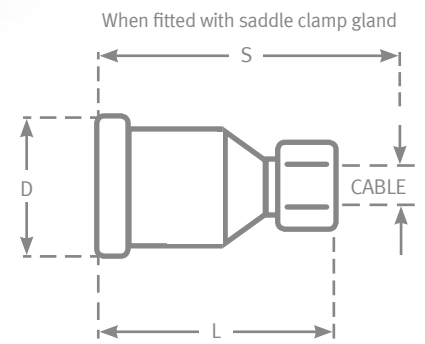
All dimensions in mm D - Diameter L - Length
